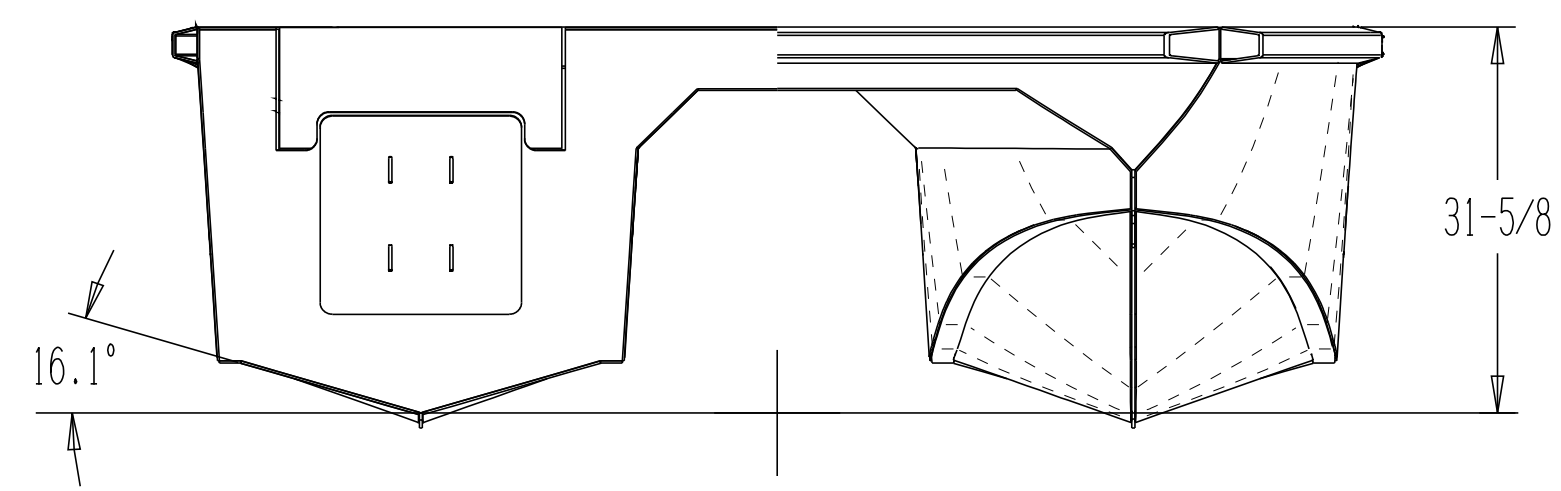
AFT VIEW
