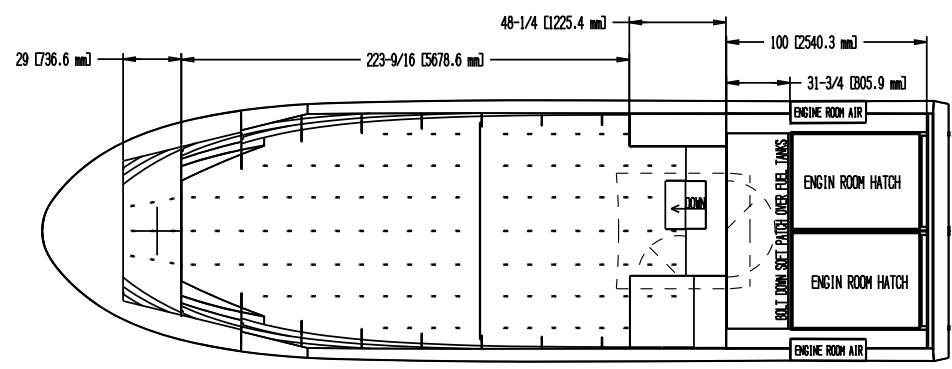
DECK PLAN
