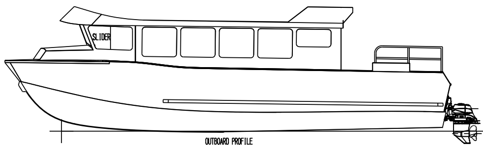
OUTBOARD PROFILE
