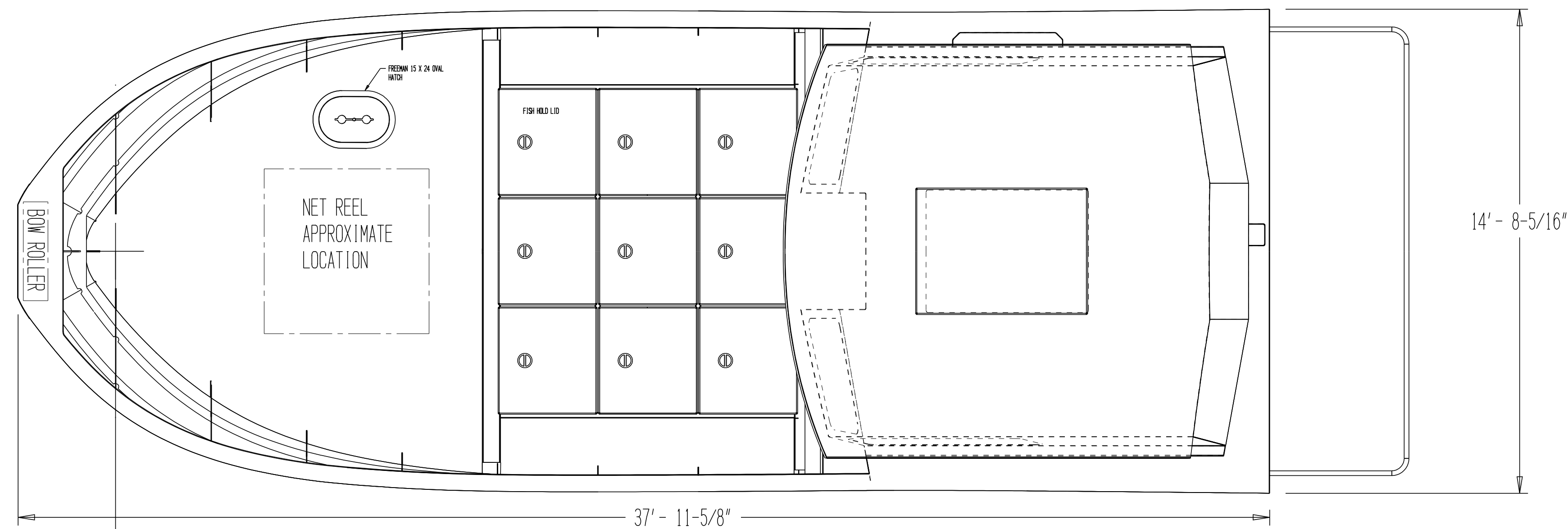
DECK PLAN
