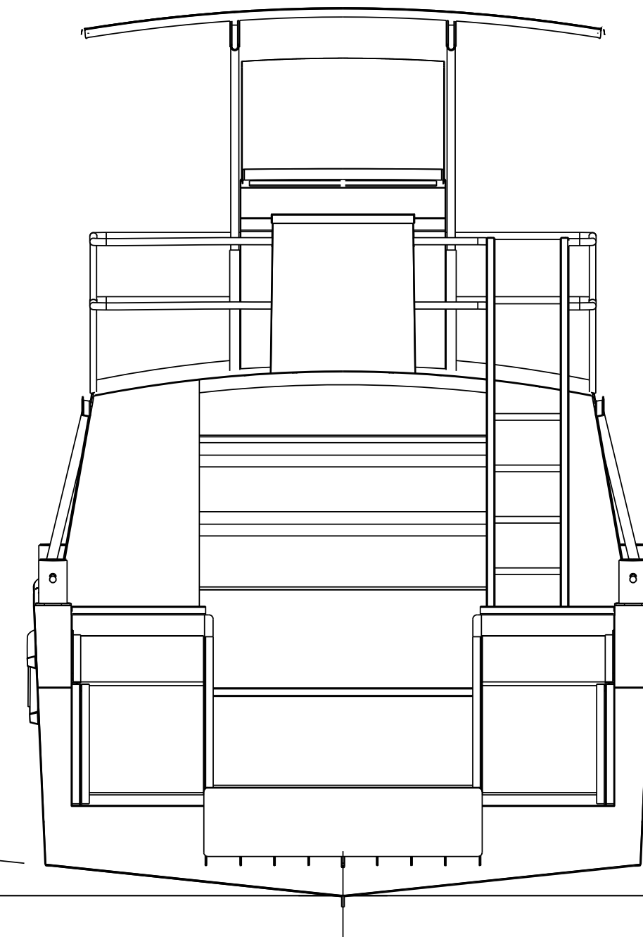
STERN VIEW
