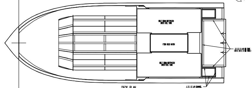
DECK PLAN
