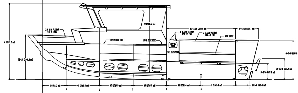
INBOARD PROFILE
