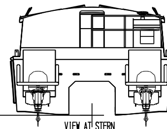
VIEW AT STERN LOOKING FORWARD
